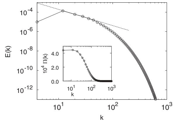
FIG. 6. Kinetic energy spectrum at the final time of the simulation. Wave number k = 8 corresponds to the confinement scale L_x . The dotted line represents the Kolmogorov scaling k^{-5/3} . Inset: Kinetic energy flux in the wave-number space.
