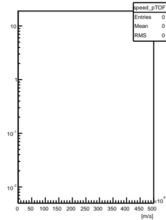
Particle speed, TOF&gt;0
