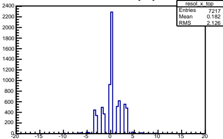
TOP X resolution [cm]
