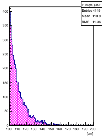
Track length, TOF&gt;0
