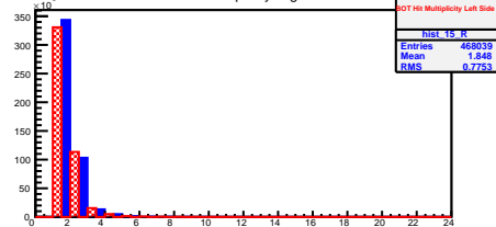
BOT Hit Multiplicity Right Side
