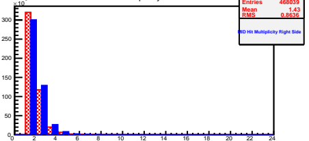
MID Hit Multiplicity Left Side
