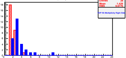
TOP Hit Multiplicity Left Side
