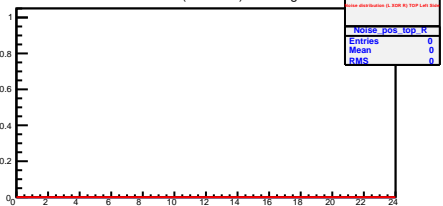
Noise distribution (L XOR R) TOP Right Side
