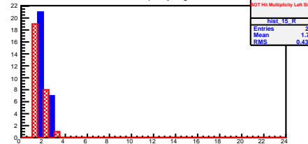
BOT Hit Multiplicity Right Side
