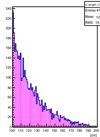
Track length, TOF&lt;0
