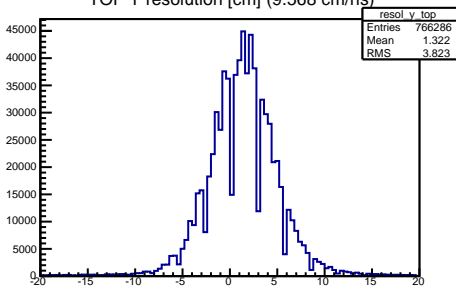
TOP Y resolution [cm] (9.568 cm/ns)
