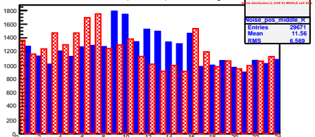
Noise distribution (L XOR R) MIDDLE Right Side
