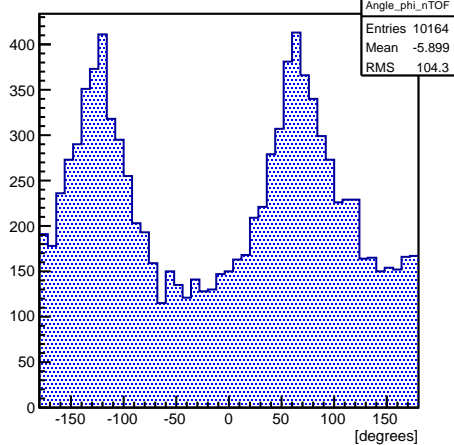
Azimuthal angle \phi , TOF<0
