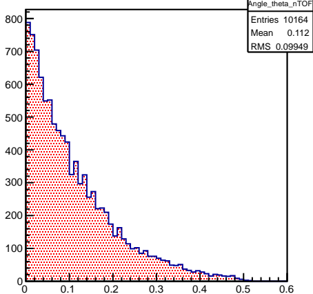
1-cos( \theta ), TOF<0
