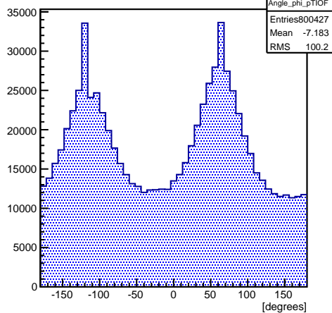
Azimuthal angle \phi , TOF>0
