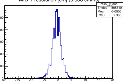
MID Y resolution [cm] (9.568 cm/ns)
