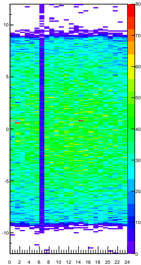
BOT Hits profile plot
