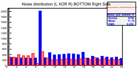
Noise distribution (L XOR R) BOTTOM Right Side
