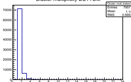
Cluster multiplicity BOTTOM
