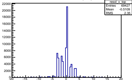
TOP X resolution [cm]
