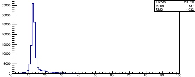
Middle-Left Width [ns]
