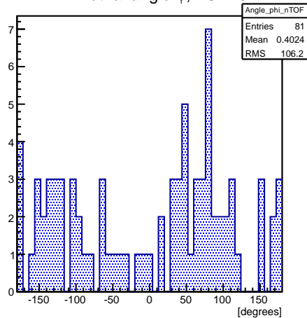
Azimuthal angle \phi , TOF<0
