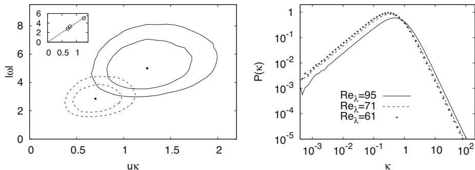
Figure 7. Left: contour plots of the 90% and 80% levels of the joint pdf of curvature angular velocity and angular velocity for Reynolds numbers Re_\lambda = 61 and Re_\lambda = 95 respectively. The inset also includes data for Re_\lambda = 71 and suggests the linear relation (28) between the maxima. Right: Pdfs of curvature at different Re_\lambda . A shift of the maximum towards larger values can be observed, as for u\kappa , at increasing Re_\lambda , while the shape of the distribution is preserved.
