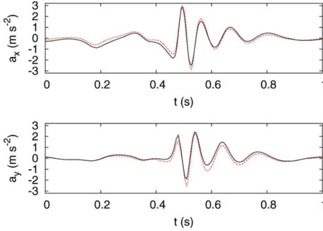
Figure 2. x -component (top) and y -component (bottom) of the acceleration of one particle computed from numerical simulations at Re_\lambda = 200 (black line) together with the acceleration estimated from the x - and y -component of the orientation vector, i.e. a_x = gp_x , a_y = gp_y see (4), of a geotropic particle with v_0 = 6 \text{ mm s}^{-1} corresponding to a displacement h = 0.5 \text{ mm} .
