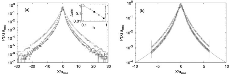
Figure 4. PDFs of acceleration in one horizontal direction for Re_\lambda = 200 (a) and Re_\lambda = 400 (b). Estimates obtained according to (2) ( X = gp_x , symbols) are compared with fluid acceleration ( X = a_x , line). Three values of particle bias were used, which rescaled on experimental values correspond to h = 0.1 mm (circles), 0.2 mm (triangles) and 0.5 mm (squares). By comparison, it is evident that the intermediate value gives a good estimate at higher Re_\lambda but is not satisfying at the lower one (see the text). In (b) the value of g (vertical lines) marks the upper cut-off for measurable accelerations. In the inset of (a): relative error on the estimate of \sigma = \sqrt{\langle a_x^2 \rangle} as a function of h , for Re_\lambda = 200 , \Delta\sigma = g\sqrt{\langle p_x^2 \rangle} - \sigma .
