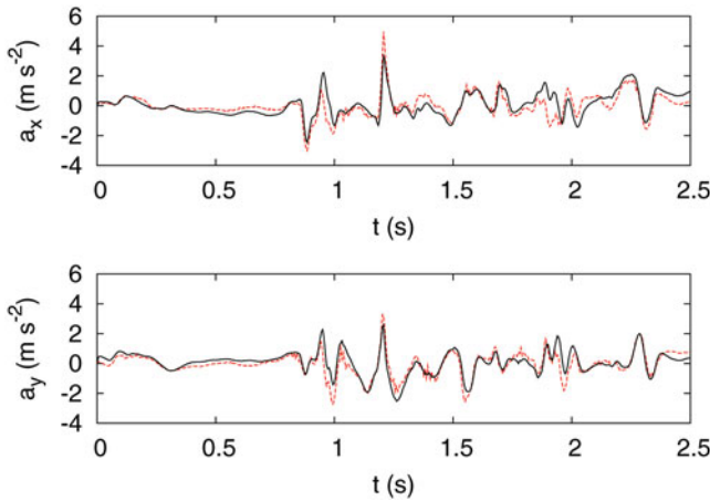
Figure 3. The same of Figure 2 for a geotropic trajectory with h = 0.2 \text{ mm} and v_0 = 15 \text{ mm s}^{-1} in a turbulent flow at Re_\lambda = 400 .
